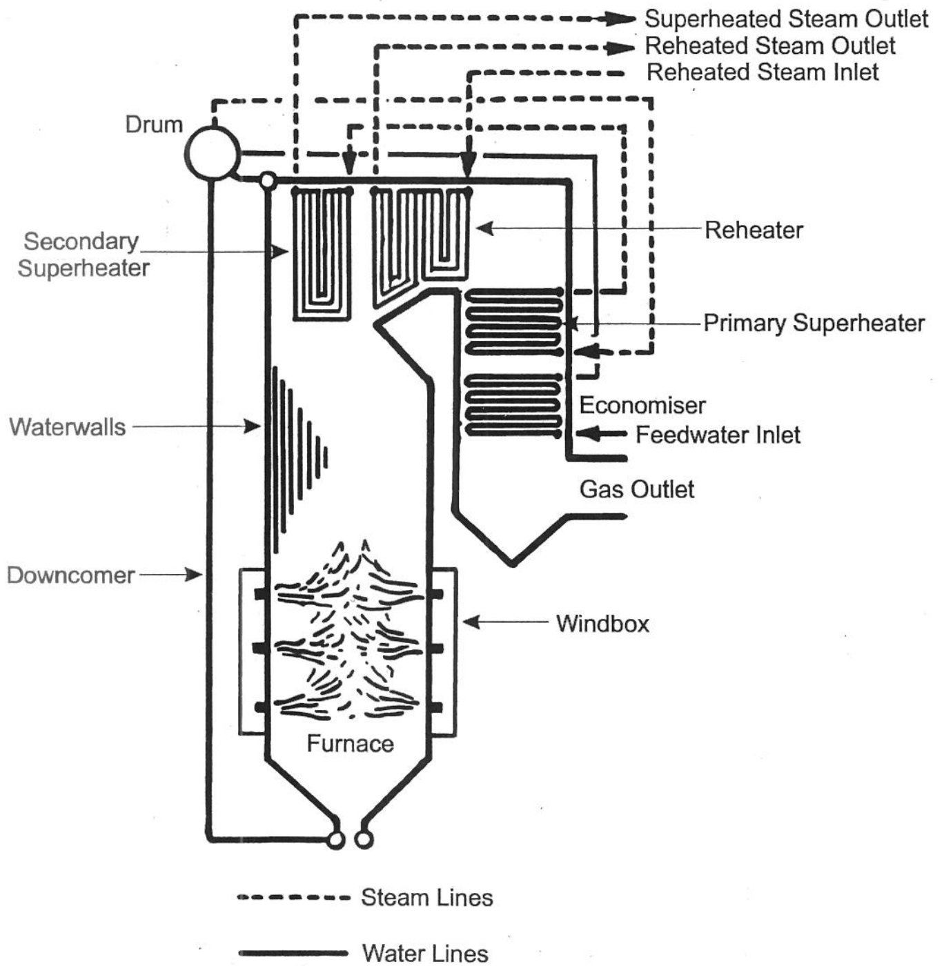
Figure 1 Typical boiler heat absorption components
