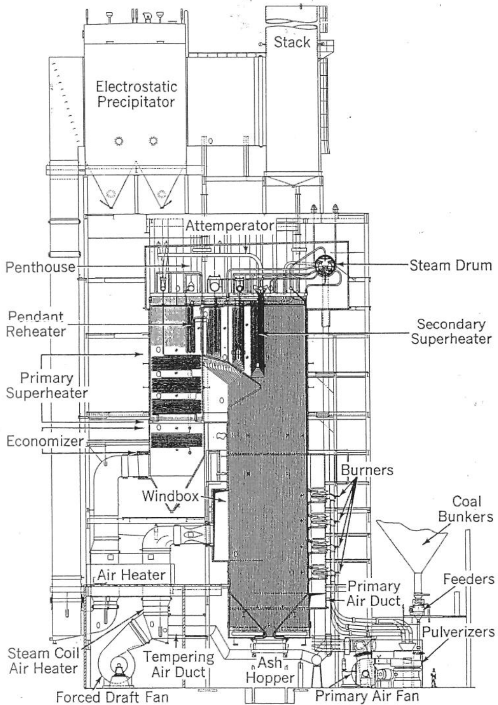
Fig. 2 Radiant boiler for pulverized coal.
